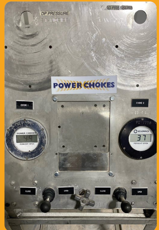
Figure 2: Slimline remote panel dual choke
